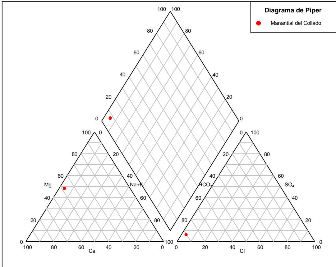
Figura 13. Diagrama Piper - Hill - Langelier.
